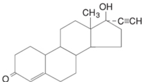
Norethindrone C 20 H 26 O 2 Molecular Weight: 298.4
