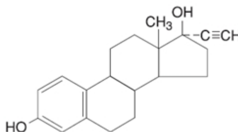
Ethinyl Estradiol C 20 H 24 O 2 Molecular Weight: 296.40
